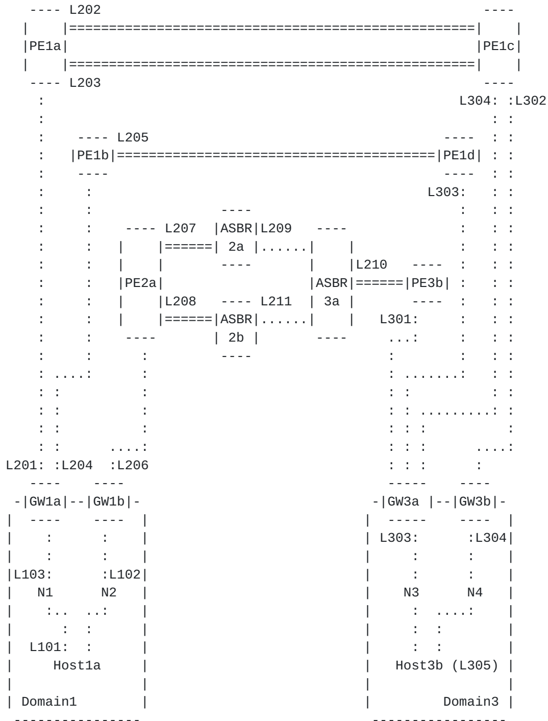
Figure 4: Tunnels and Labels in Example Configuration
