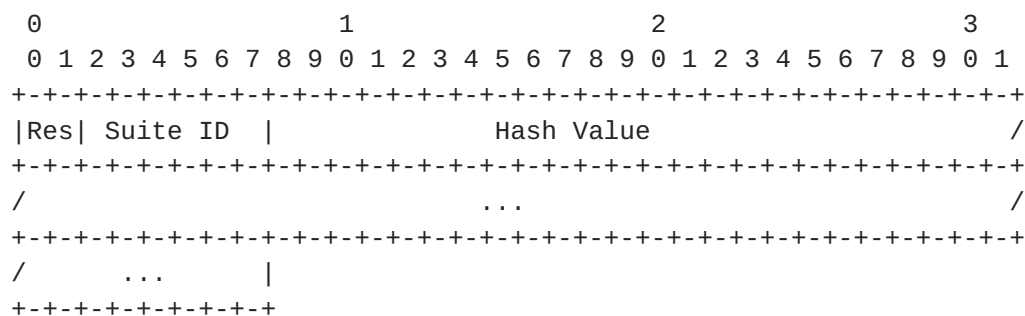
Figure 3: Binary Name Format
