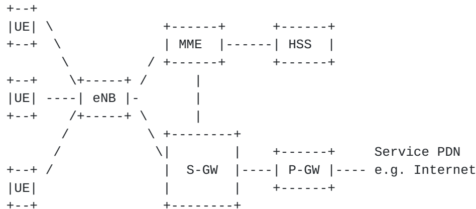
Figure 3: 3GPP network architecture
