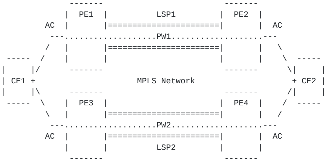
Figure 27 : Path-Diverse Pseudowires With Disjoint PEs
