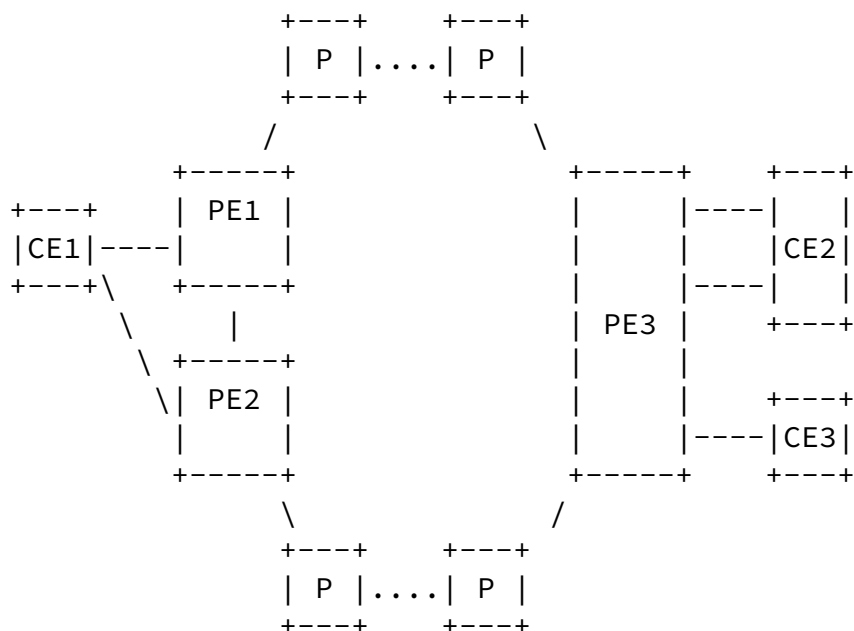
Figure 1 Overlay Reference Diagram
