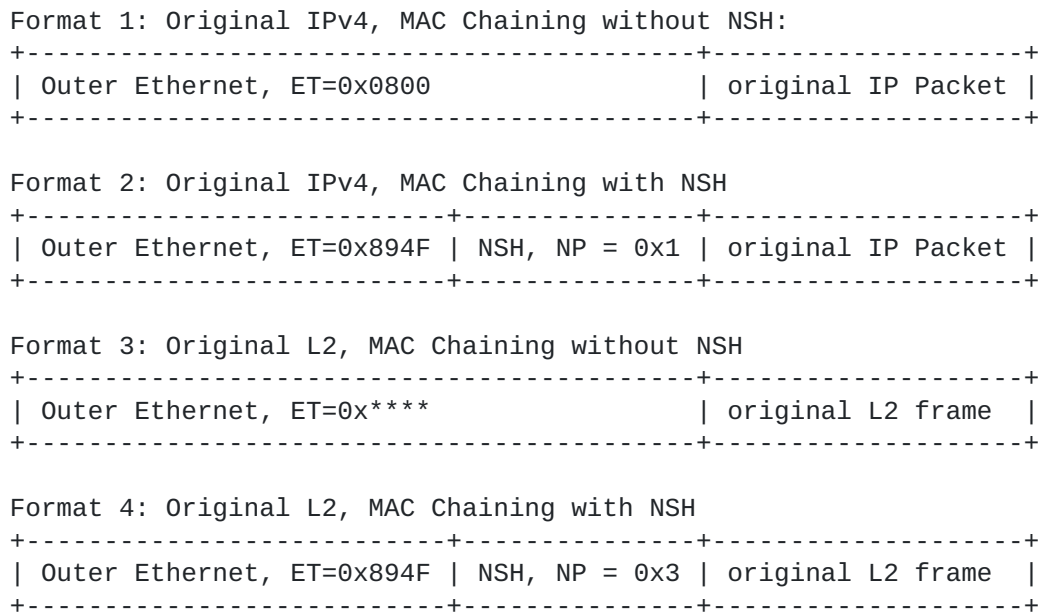
Figure 3 MAC Chaining Formats for IPv4 and L2 Service Packets
