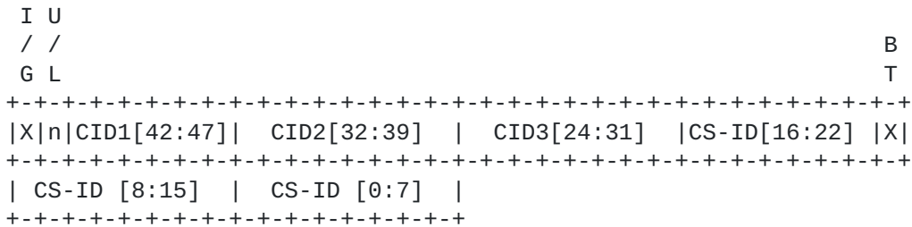
Figure 4 MAC Chaining Ethernet MAC address Format
