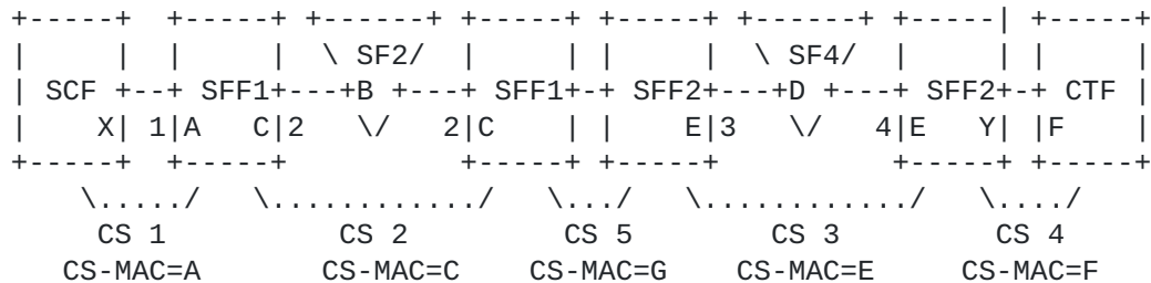
Figure 2 MAC Chain Segments Addressing
