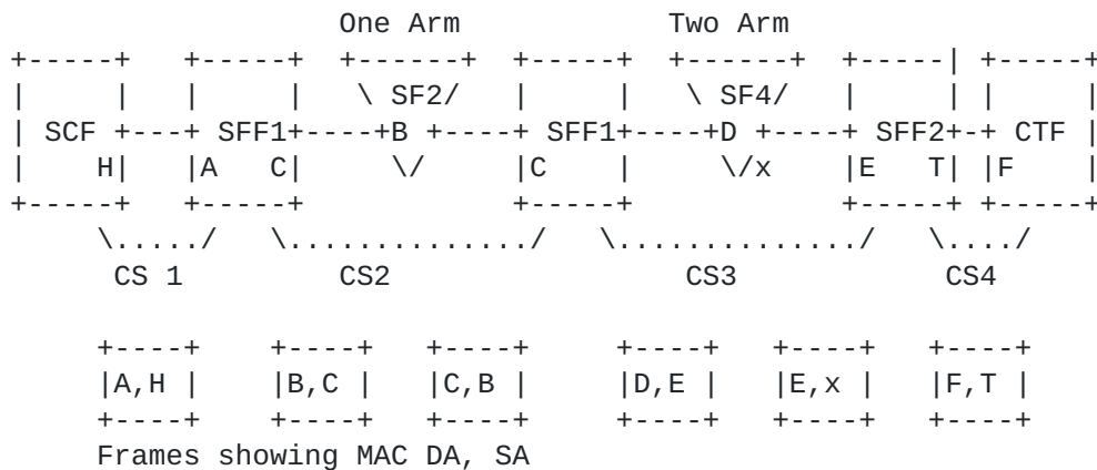
Figure 6 MAC Service Chain Example
