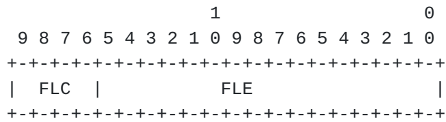
Figure 2: Structured Flow Label Format
