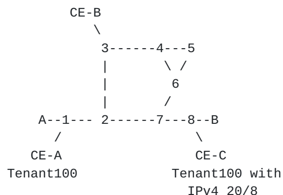
Figure 1: Reference topology
