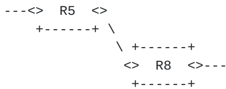
Figure 3: Clusters Example
