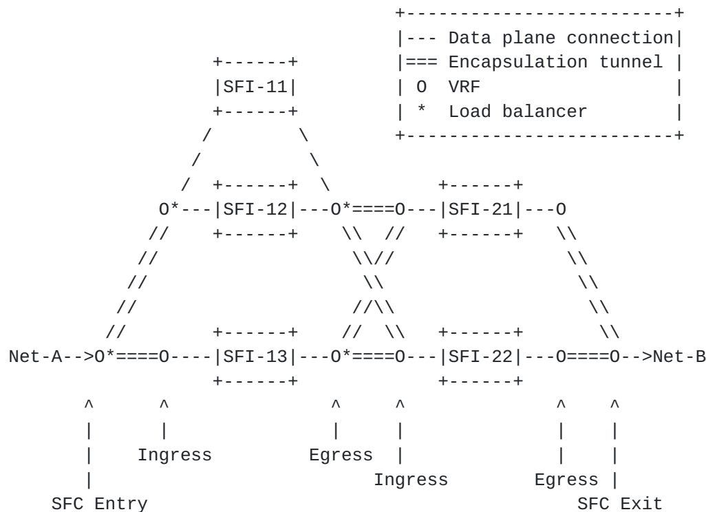
Figure 8 - Load Balancing across SF Instances
