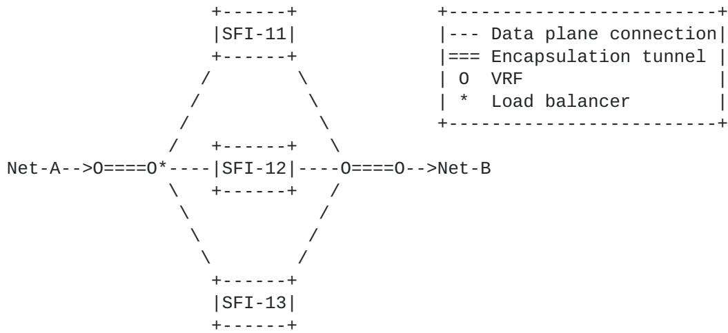
Figure 7 - Ingress VRF Load Balancing across SF Instances Connected to the Same VRF
