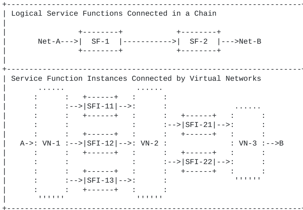
Figure 3 - Service Functions Are Composed of SF Instances Connected Via Virtual Networks
