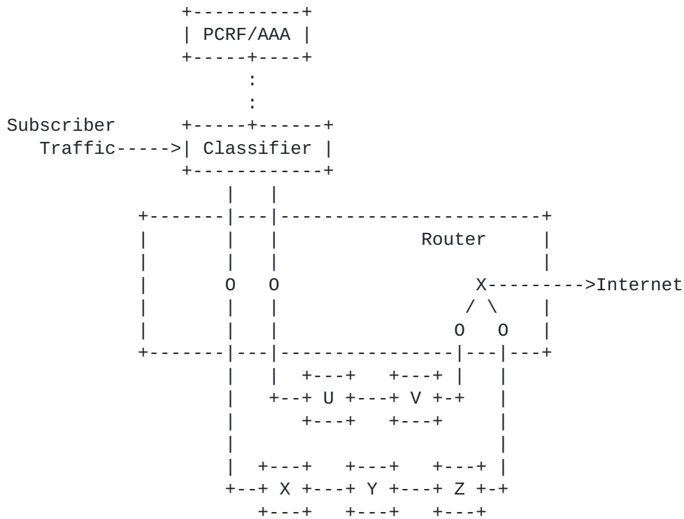
Figure 9 - Subscriber/Application-Aware Steering with a Classifier
