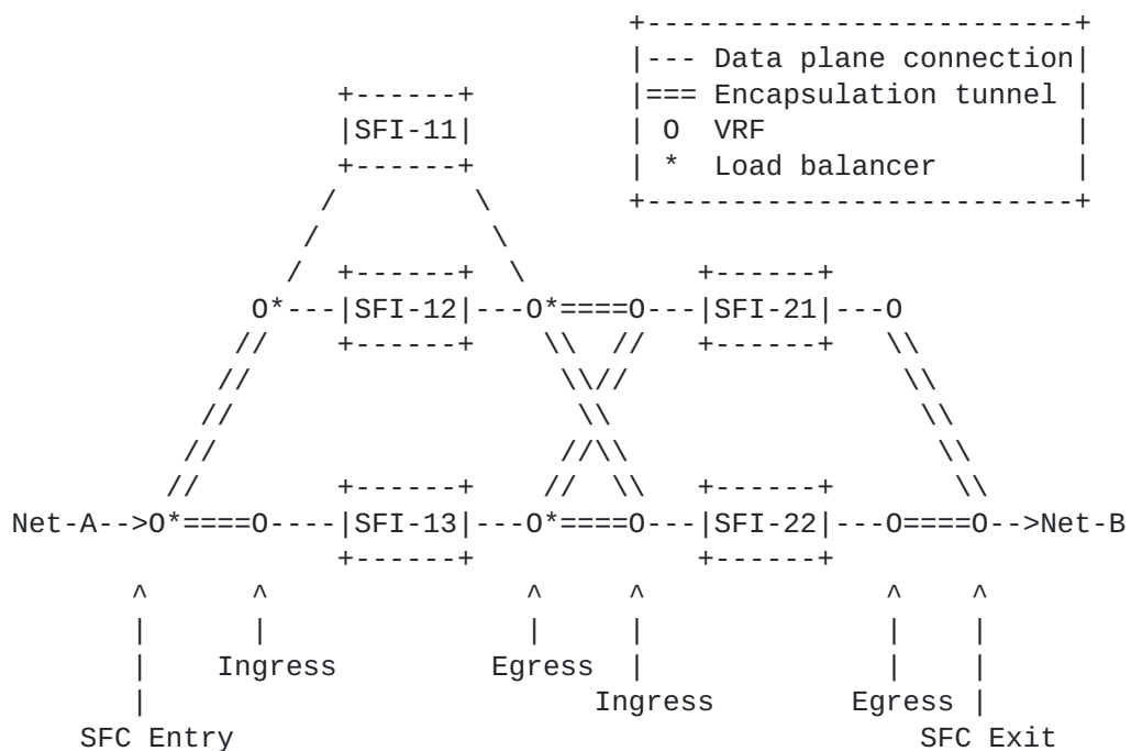
Figure 8 - Load Balancing across SF Instances
