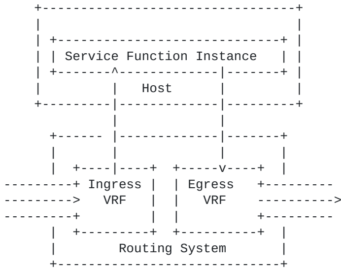
Figure 4 - Ingress and Egress VRFs for a Physical Routing System and Physical SF Instance
