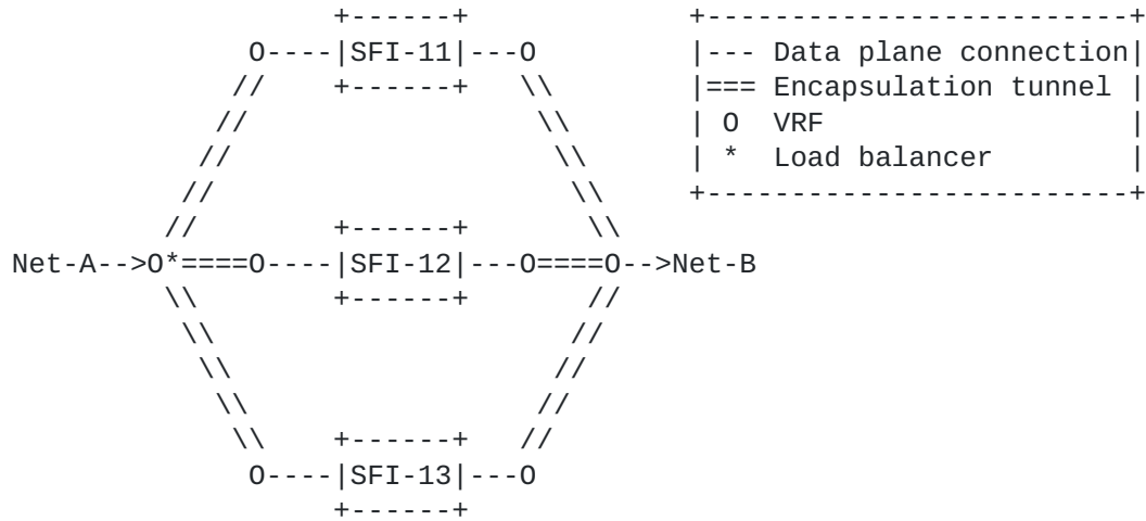
Figure 6 - Egress VRF Load Balancing across SF Instances Connected to Different VRFs
