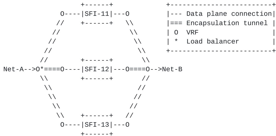
Figure 6 - Egress VRF Load Balancing across SF Instances Connected to Different VRFs
