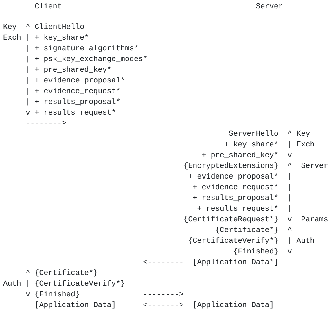
Figure 11: Attestation Message Overview.
