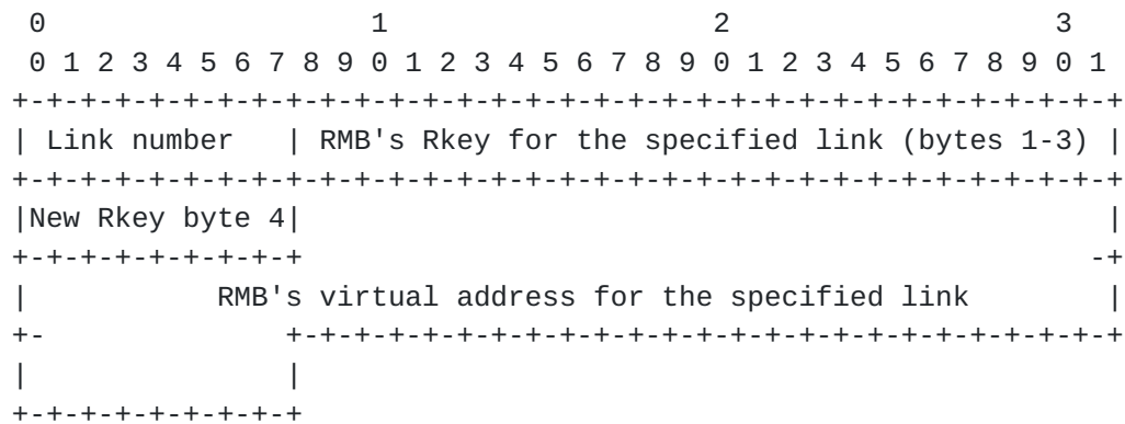
Figure 37 Format of link number/Rkey pairs
