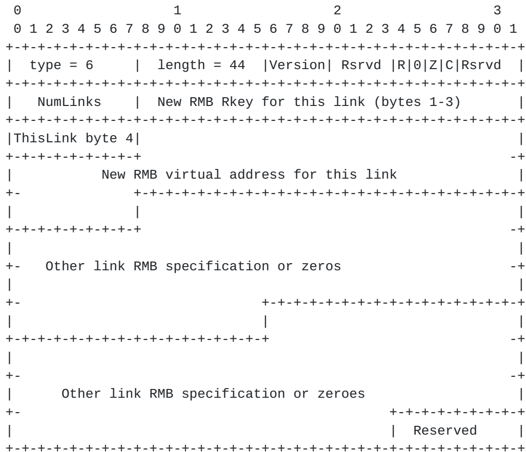
Figure 36 CONFIRM RKEY LLC message format
