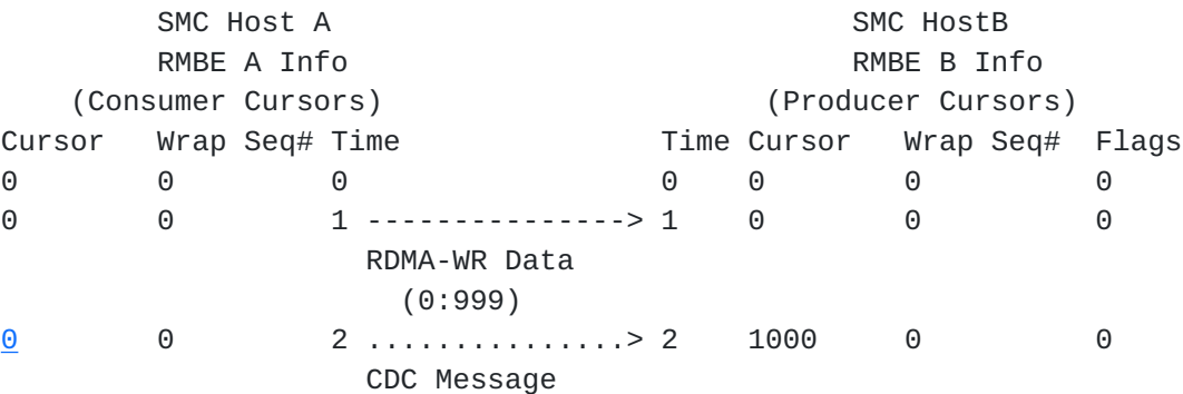
Figure 16 Scenario 1: Send flow, window size unconstrained
