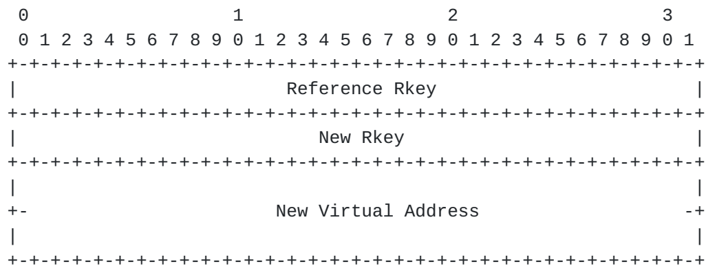
Figure 34 Rkey/RToken pair format
