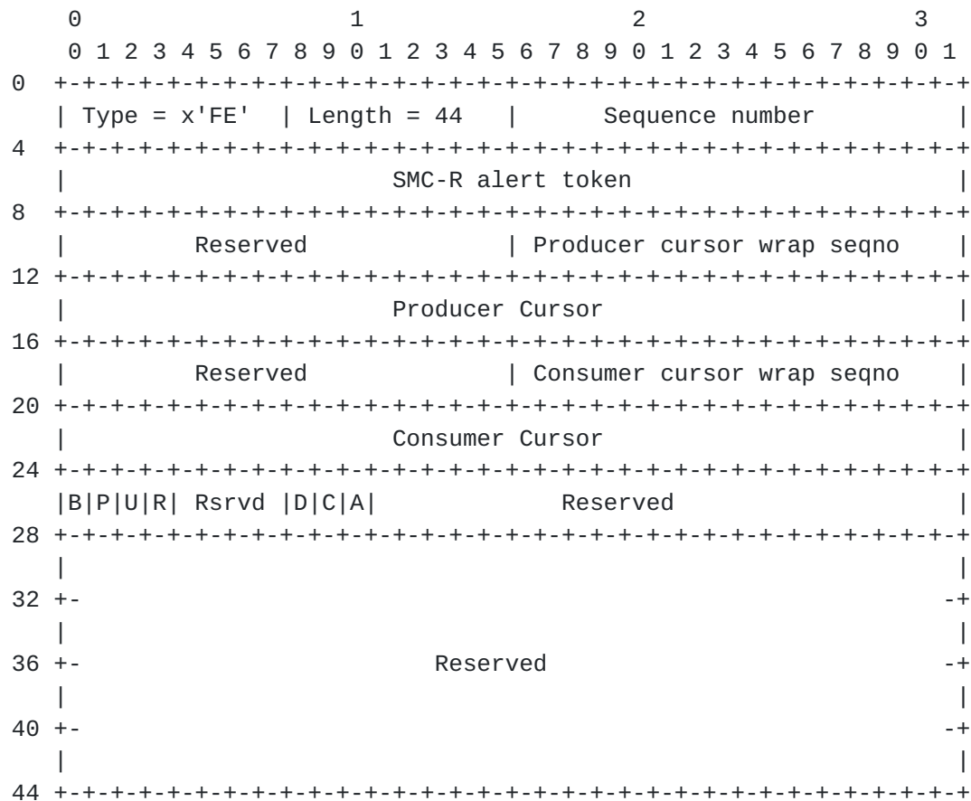
Figure 39 Connection Data Control (CDC) Message Format
