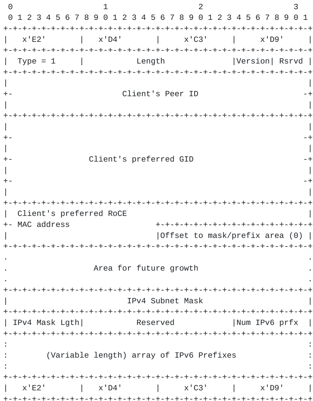
Figure 26 SMC Proposal1 CLC message format
