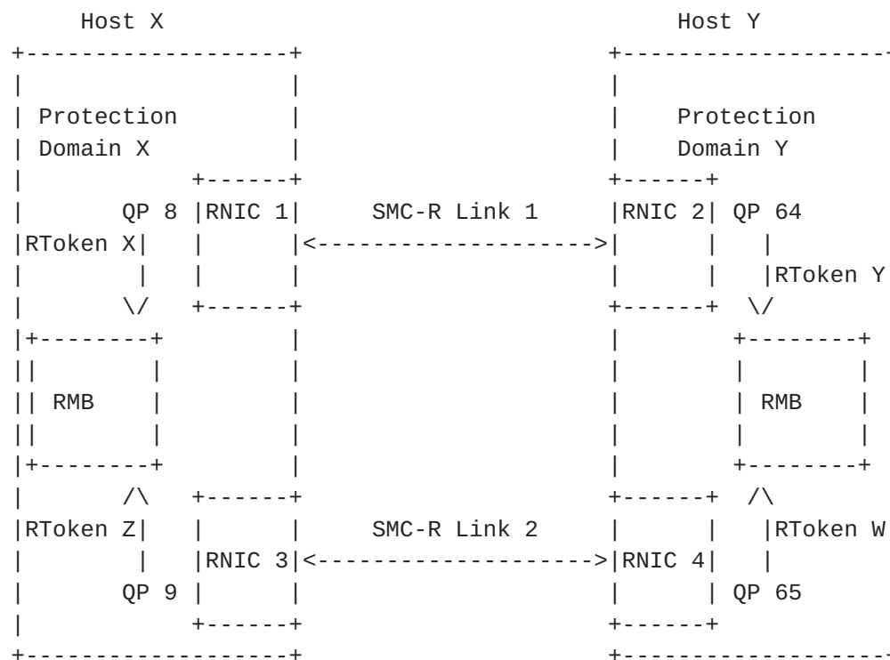
Figure 5 Symmetric SMC-R links
