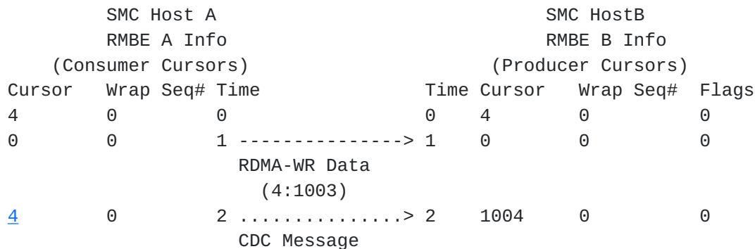
Figure 16 Scenario 1: Send flow, window size unconstrained
