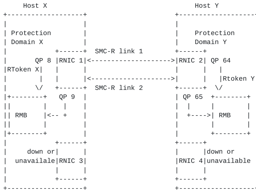
Figure 7 SMC-R parallel links (not supported)
