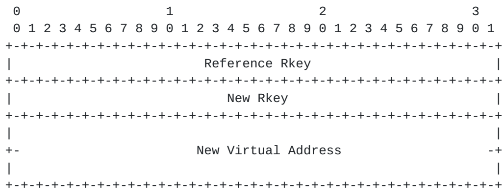
Figure 34 Rkey/Rtoken pair format
