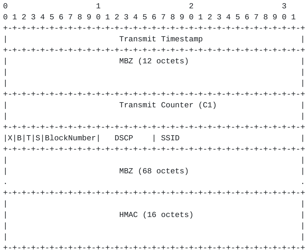
Figure 2: Session-Sender Direct Loss Measurement Probe Packet - Authenticated Mode
