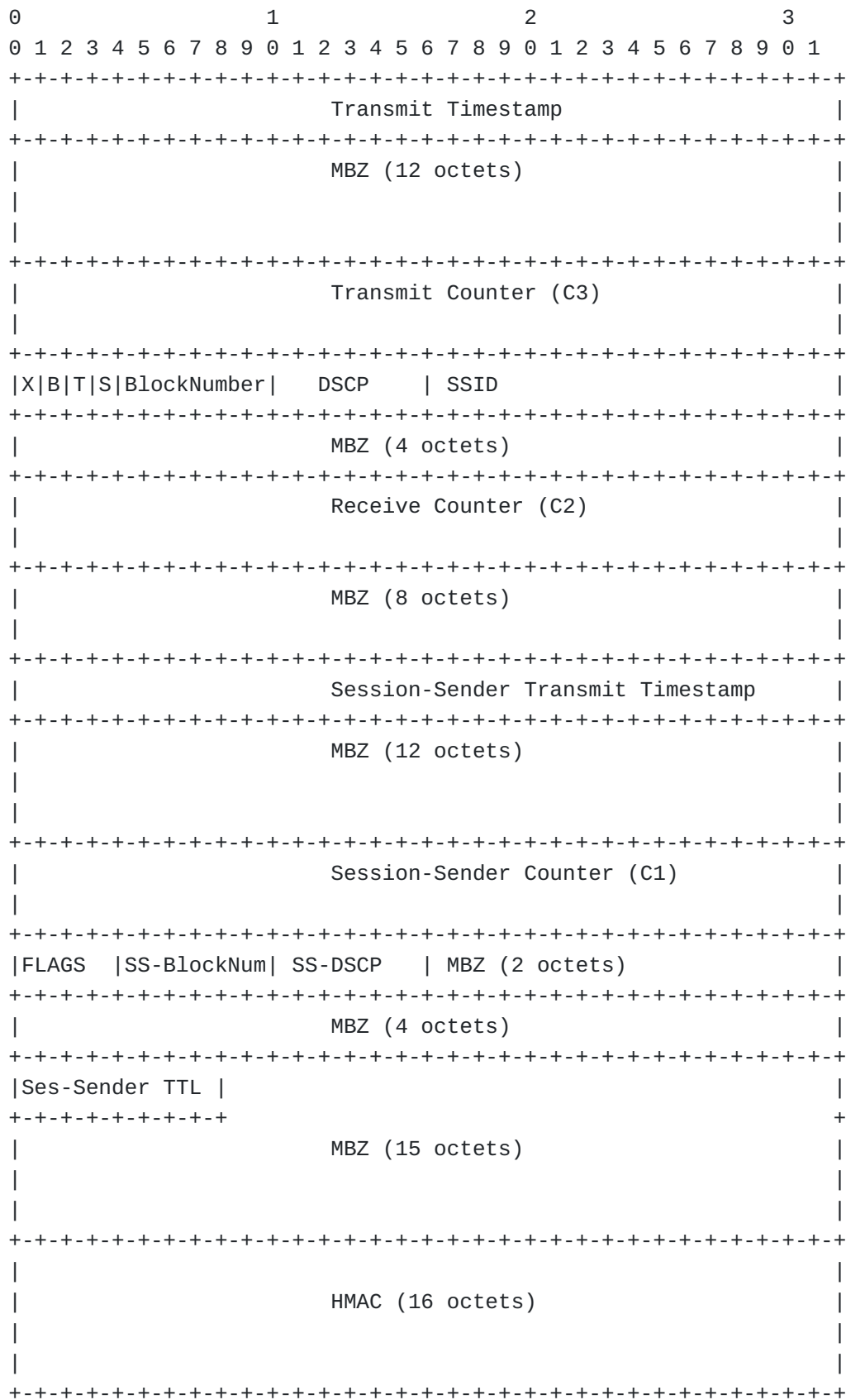
Figure 4: Session-Reflector Direct Loss Measurement Probe Packet - Authenticated Mode
