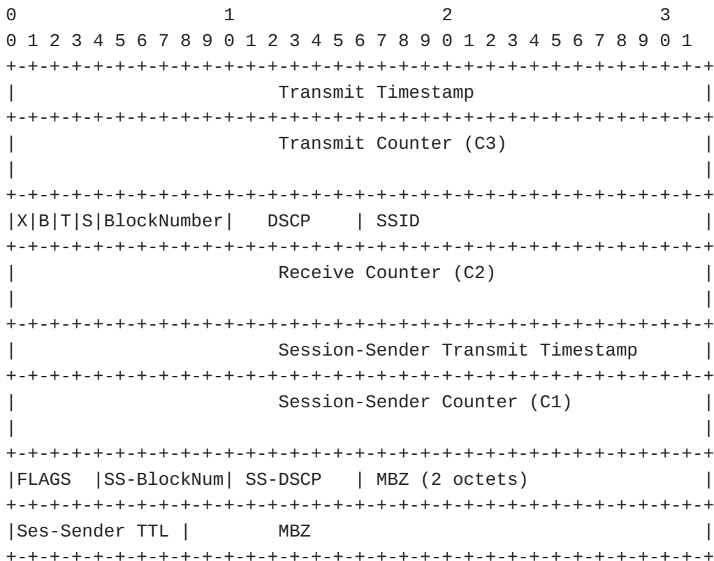
Figure 3: Session-Reflector Direct Loss Measurement Probe Packet - Unauthenticated Mode
