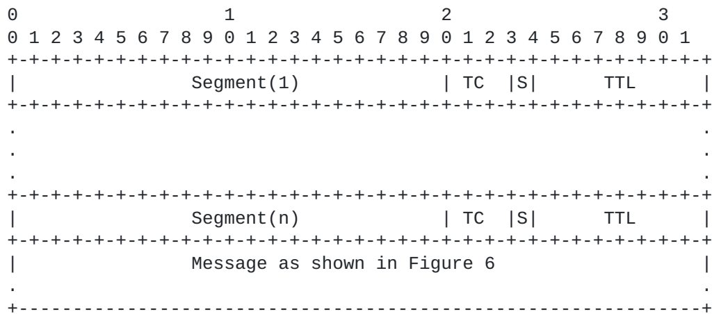
Figure 7: Example Probe Response Message for SR-MPLS Policy
