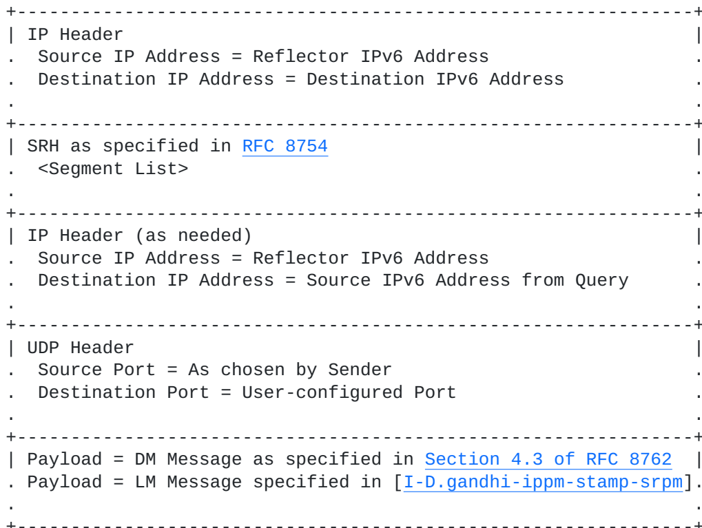
Figure 8: Example Probe Response Message for SRv6 Policy
