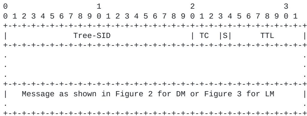
Figure 9: Example Probe Query with Tree-SID for SR-MPLS Policy
