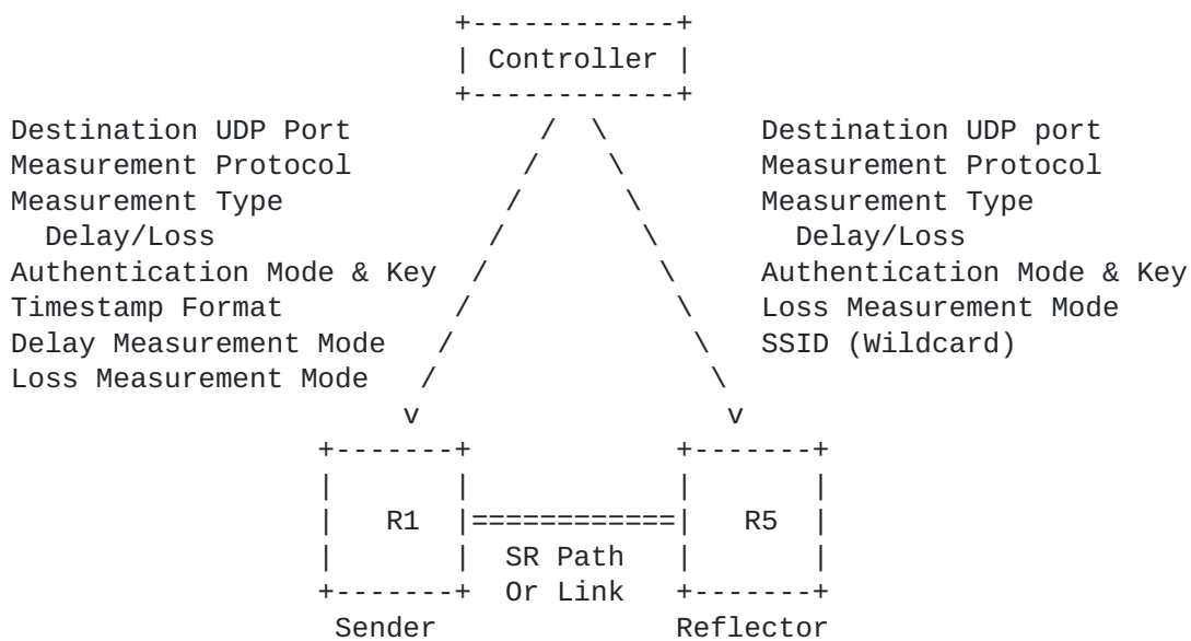
Figure 1: Example Provisioning Model
