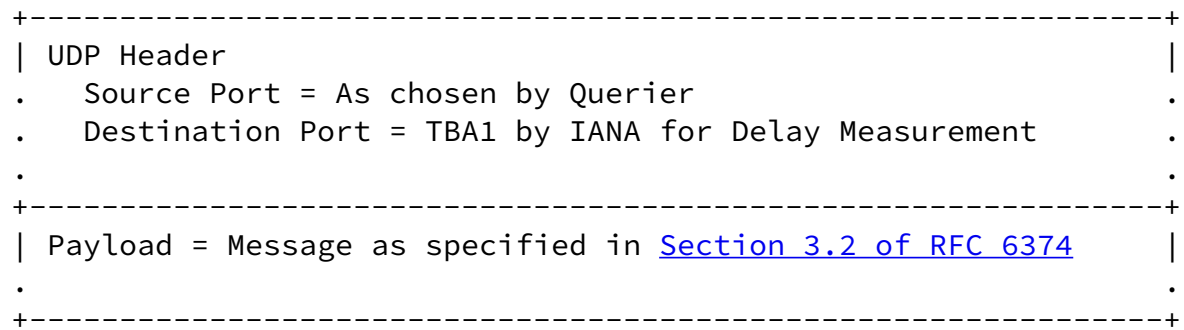
Figure 1: DM Probe Query Message
