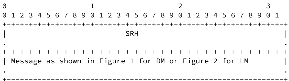
Figure 4: In-band Probe Query Message for SRv6 Policy
