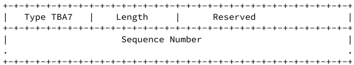
Figure 10: Sequence Number TLV
