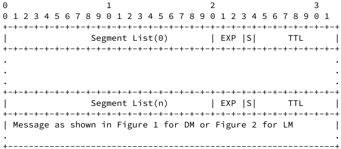
Figure 3: In-band Probe Query Message for SR-MPLS Policy
