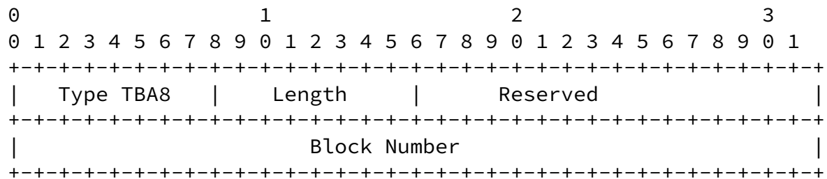
Figure 11: Block Number TLV
