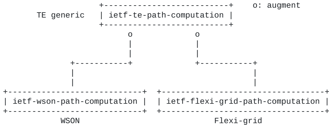
Figure 1: Relationship between WSON, Flexi-grid and TE path computation models
