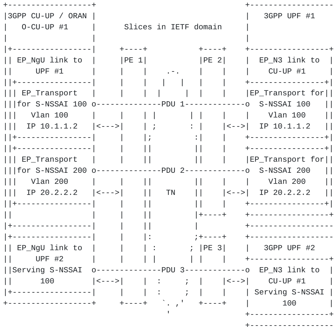
Figure 5-5 Example of CU-UP Slice in the 3GPP domain using an IETF Netwo
