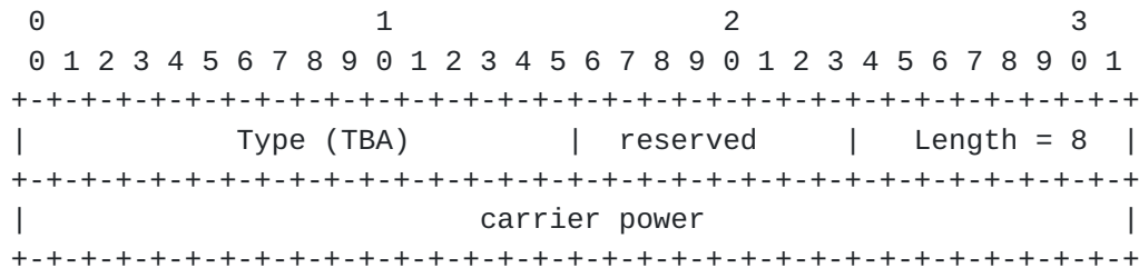
Figure 7: Carrier Power
