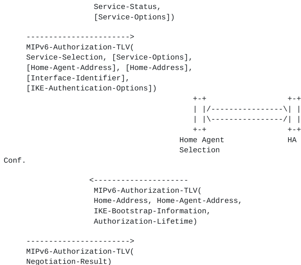
Figure 3 - MIPv6 bootstrapping procedure
