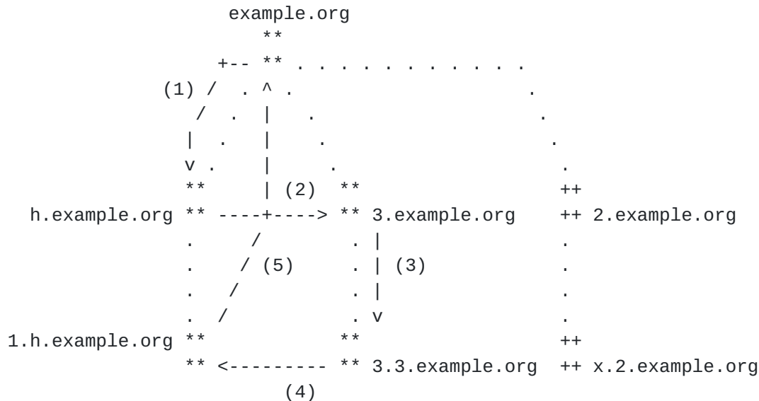
Figure 9: x.2.example.org does not exist. The five arrows represent the NSEC3 records, the ones numbered (1), (2) and (3) are the NSEC3s returned in our answer. 2.example.org is covered by (3) and x.2.example.org is covered by (4).
