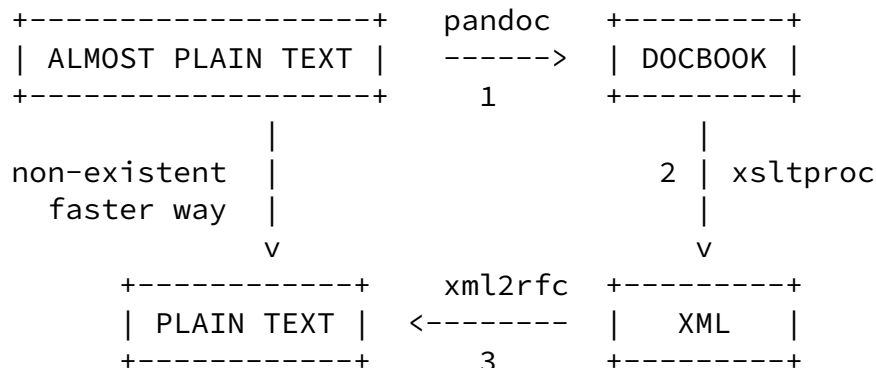
Figure 1: Attempt to justify Pandoc2rfc.
