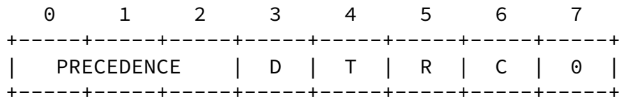
Figure 2: Type of Service field
