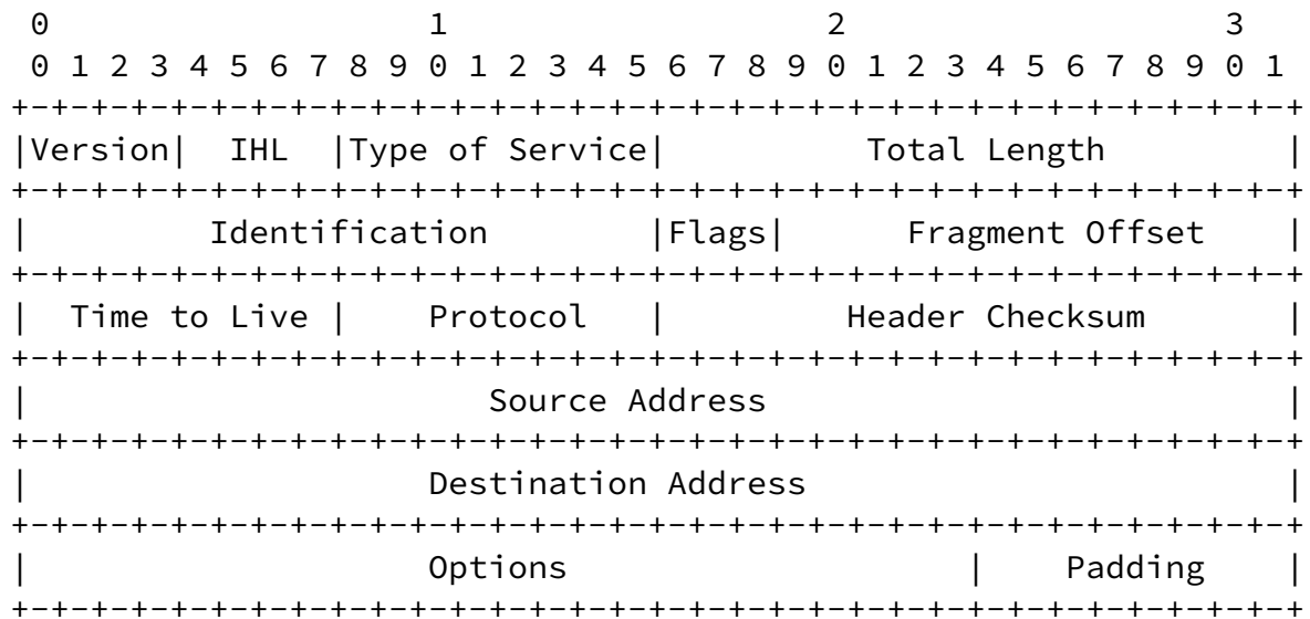
Figure 1: Internet Protocol header format
