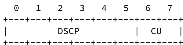
Figure 5: Structure of the DS Field
