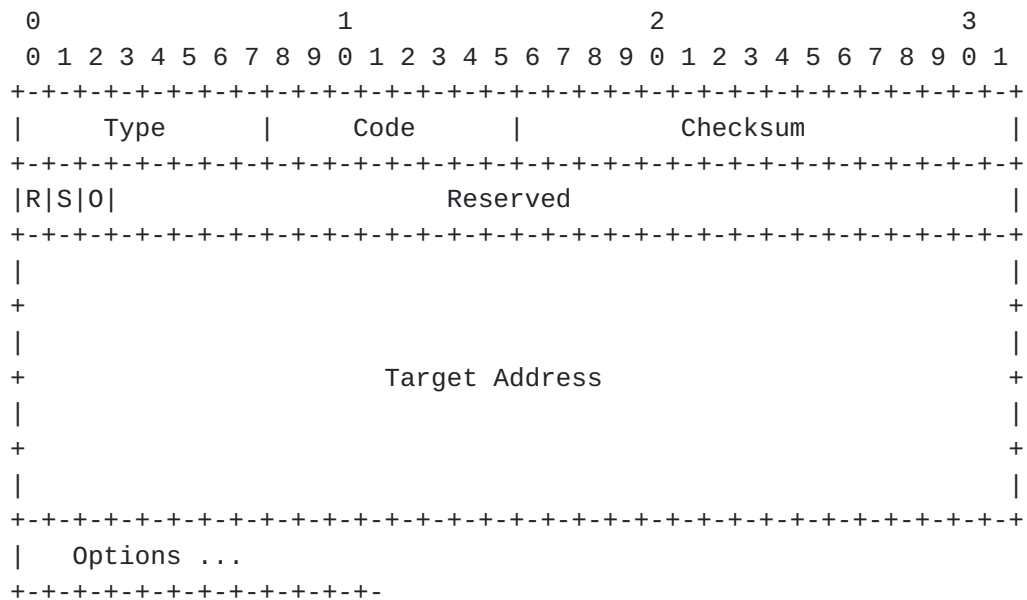
Figure 4: ICMPv6 Neighbor Advertisement message format
