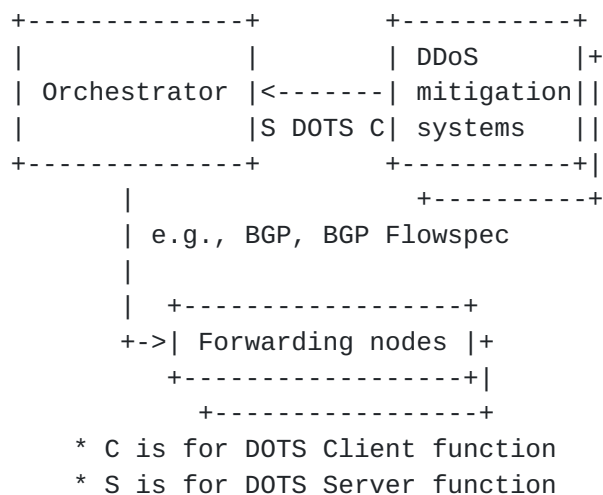
Figure 1: Component Diagram of DDoS Mitigation Offload Use Case
