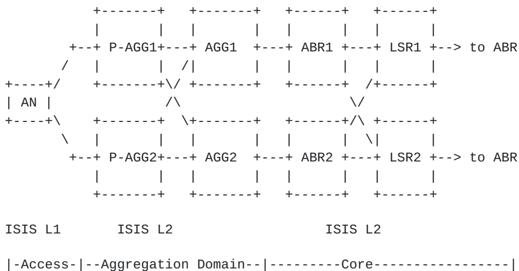
Figure 2: 5G network
