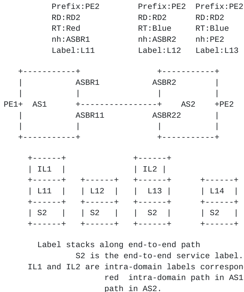
Figure 12: Translating Transport Classes across Domains
