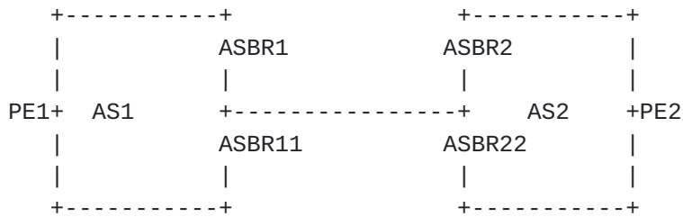
Figure 5: Network Mergers
