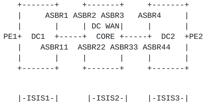
Figure 3: DCI Network
