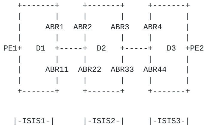
Figure 2: WAN Network
