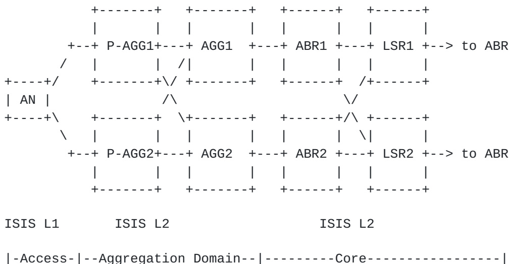
Figure 1: 5G network
