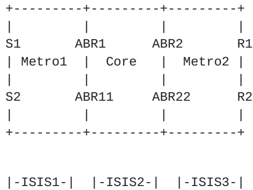
Figure 6: Multicast usecases
