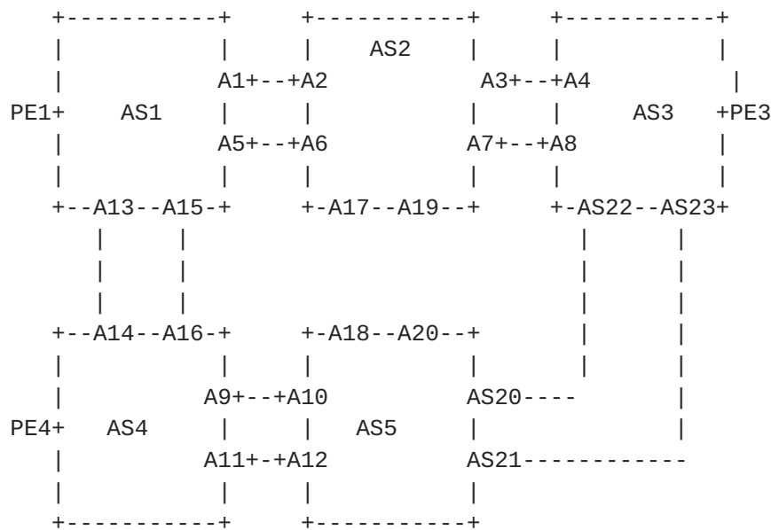
Figure 10: Multi-domain Network
