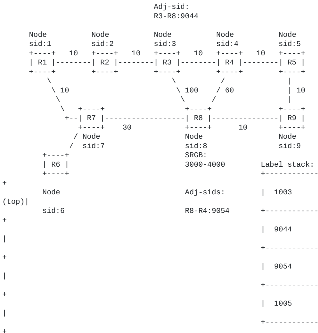
Figure 3: Explicit path using an adjacency sid. All nodes have SRGB = [1000-2000], except for R8 which has SRGB = [3000-4000].
