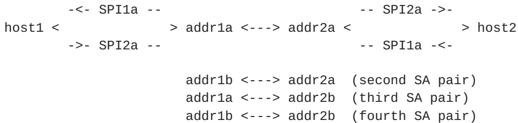
Figure 6: Dual Multihoming Case in Which Each Host Uses LOCATOR to Add a Second Address
