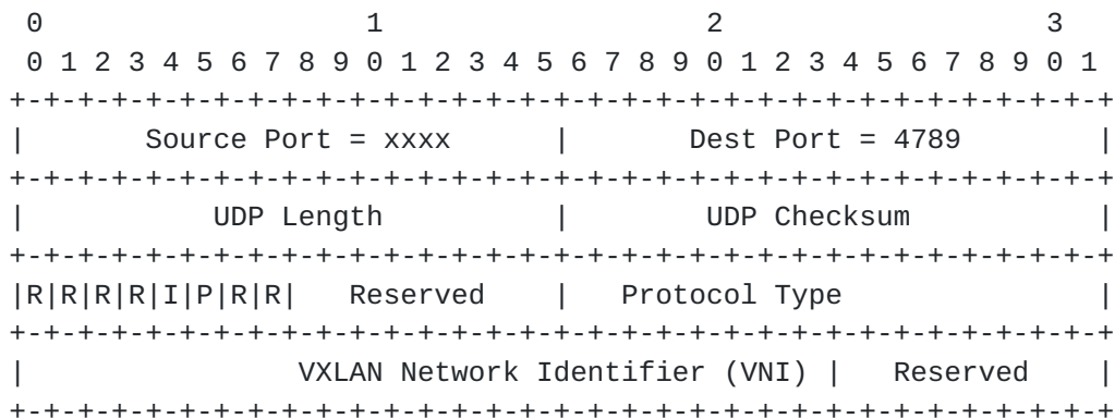
Figure 4: VXLAN with Generic Protocol Extension
