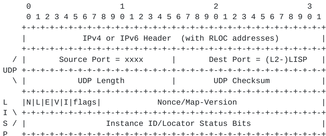
Figure 2: LISP Header
