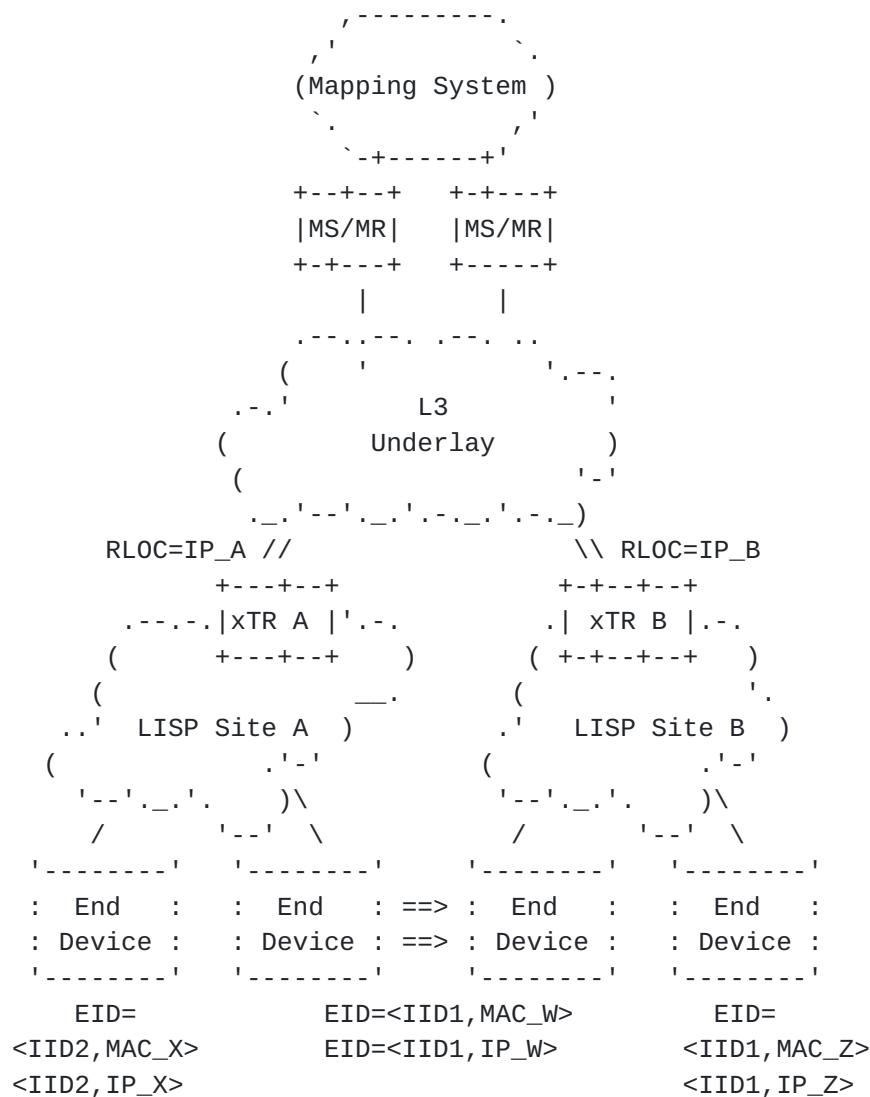
Figure 1: End System Mobility
