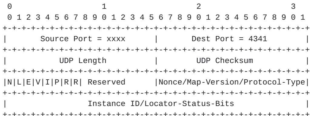
Figure 3: LISP with Generic Protocol Extension Header
