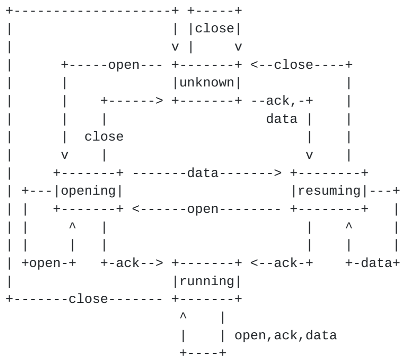
Figure 1: State transitions
