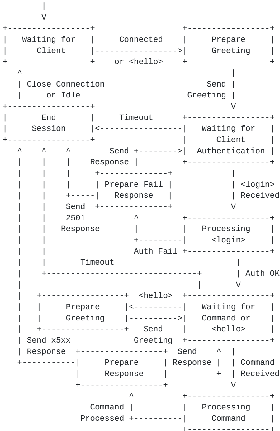
Figure 1: EPP Server State Machine
