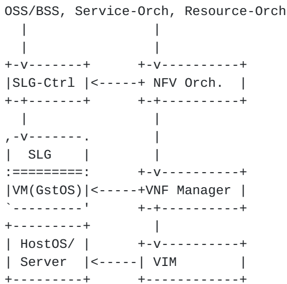
Figure 11: Position of SLG as a VM on ETSI NFV MANO
