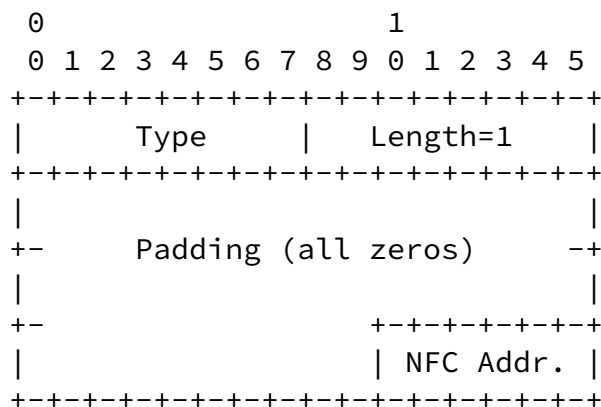
Figure 6: Unicast address mapping
