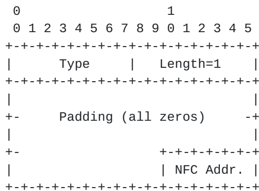
Figure 6: Unicast address mapping
