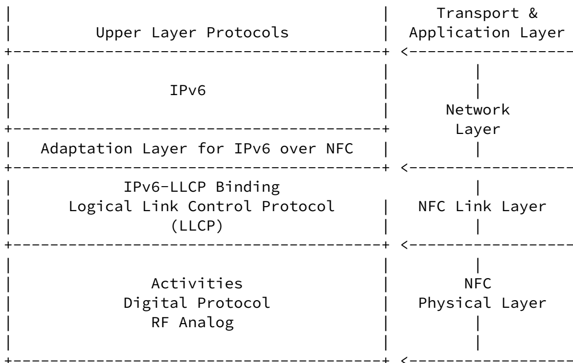
Figure 3: Protocol Stack for IPv6 over NFC
