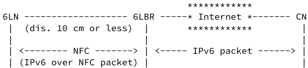
Figure 8: NFC-enabled device network connected to the Internet
