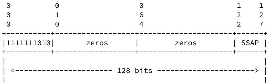
Figure 4: IPv6 link-local address in NFC
