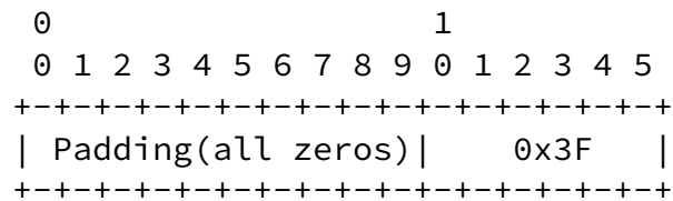
Figure 7: Multicast address mapping
