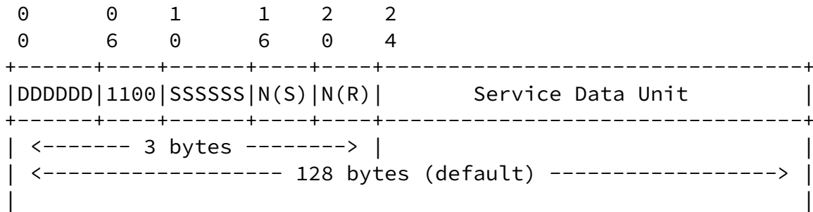
Figure 2: Format of the I PDU in NFC
