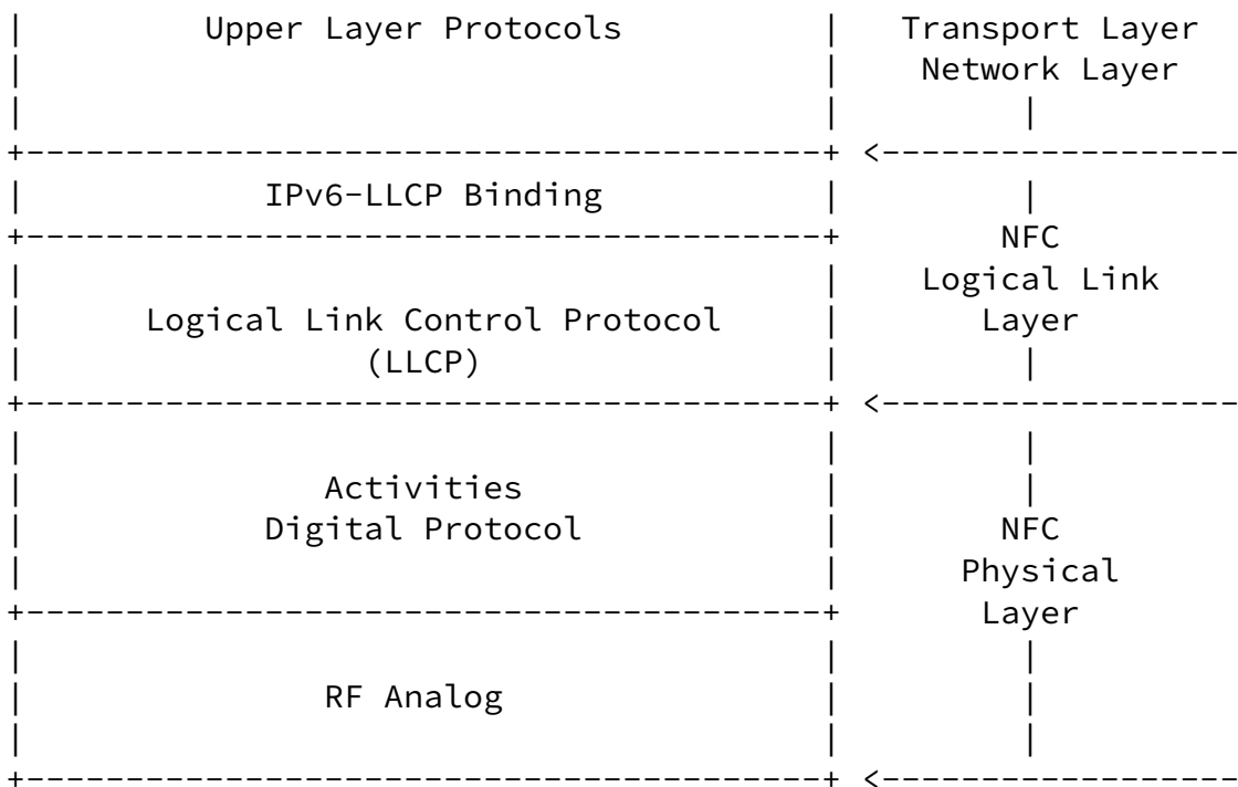
Figure 1: Protocol Stack of NFC
