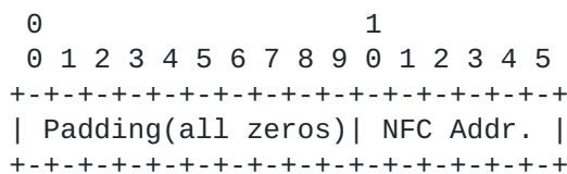
Figure 5: NFC short address format
