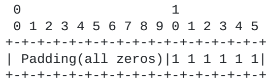
Figure 7: Multicast address mapping
