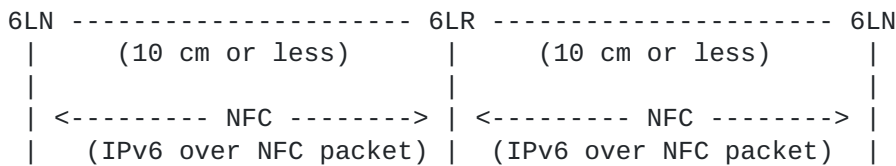
Figure 9: Isolated NFC-enabled device network
