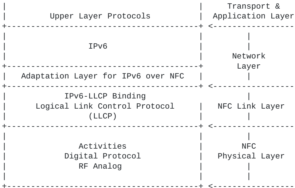
Figure 3: Protocol Stack for IPv6 over NFC
