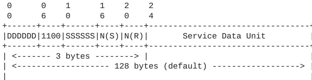
Figure 2: Format of the I PDU in NFC
