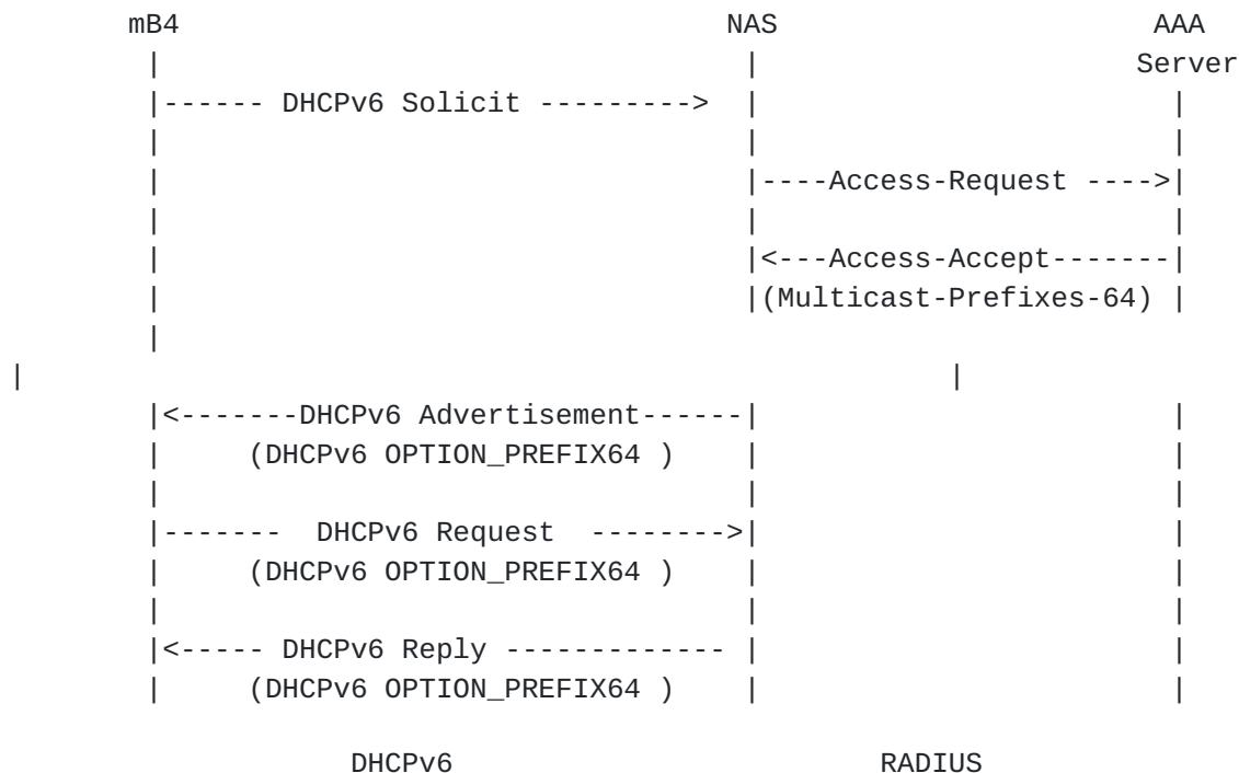
Figure 1: RADIUS and DHCPv6 Multicast-Prefixes-64 attribute Message Flow for a IP Session
