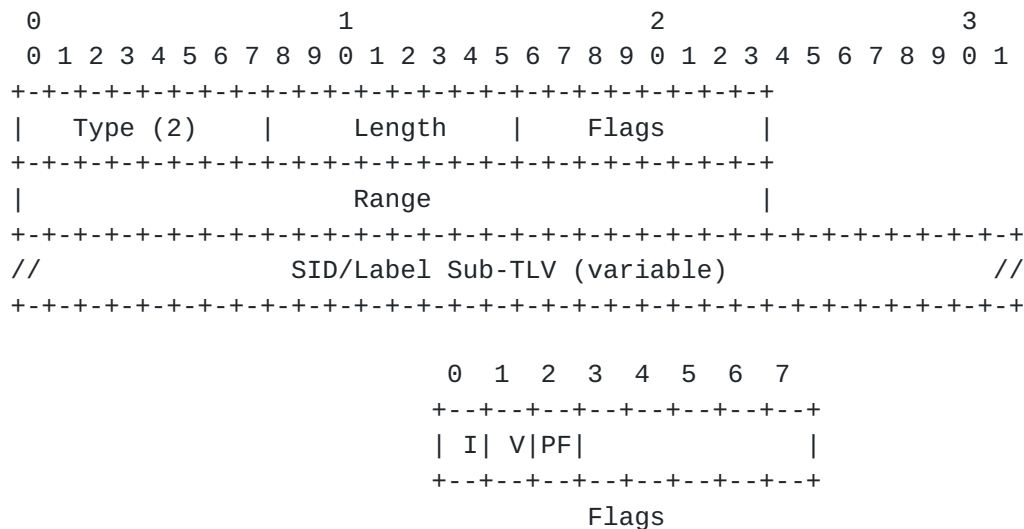
Figure 7: SR Capabilities sub-TLV
