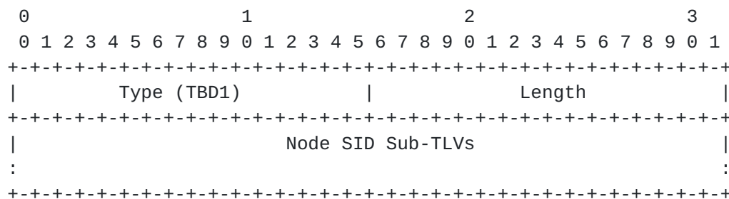
Figure 2: OSPF Proxy Node SIDs TLV
