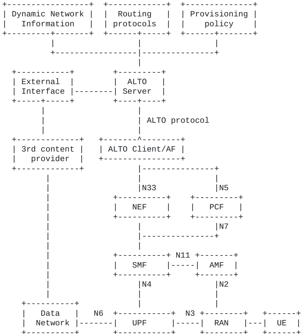
Figure 5-1: Convergence of 5G network architecture and IETF ALTO
