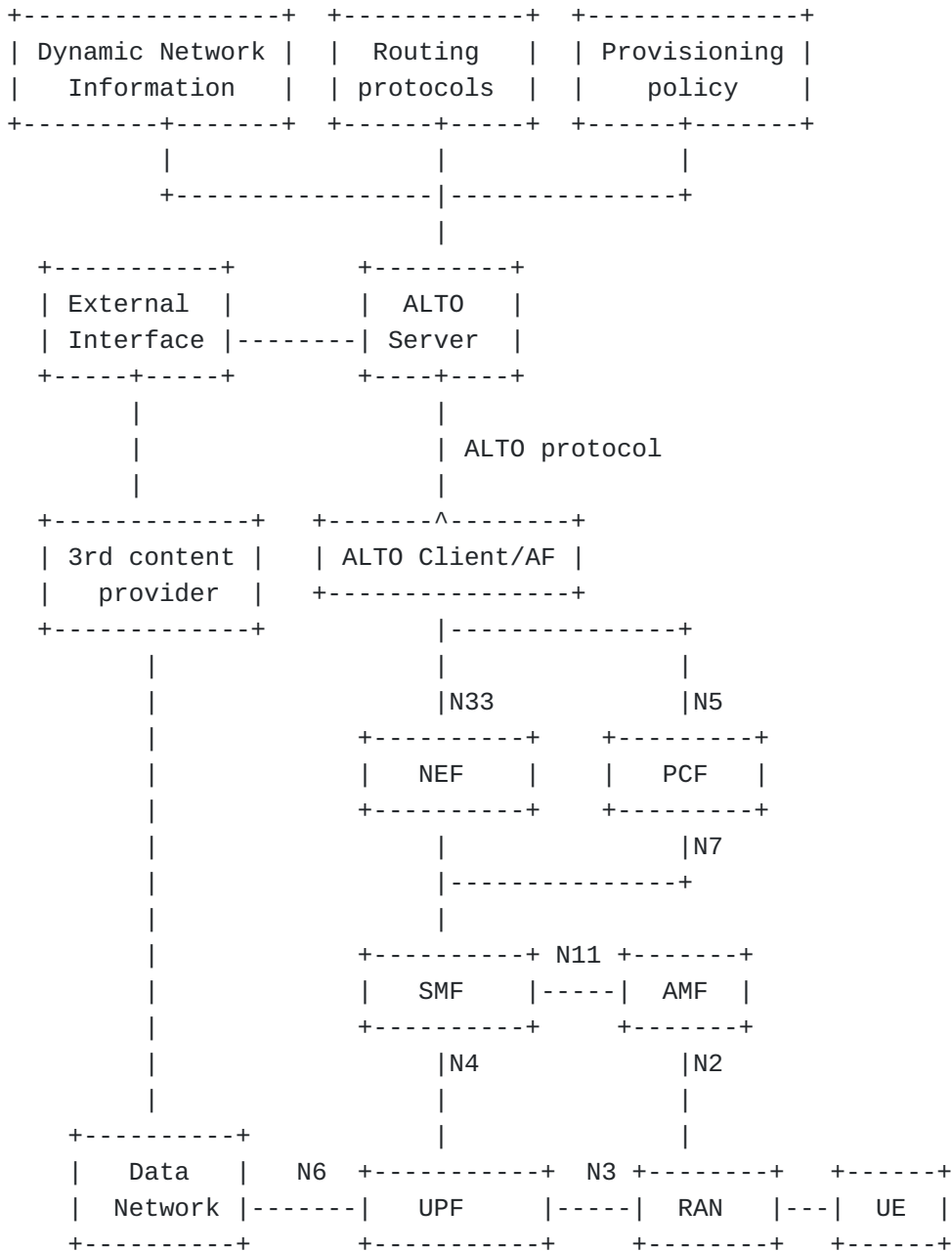
Figure 5-1: Convergence of 5G network architecture and IETF ALTO
