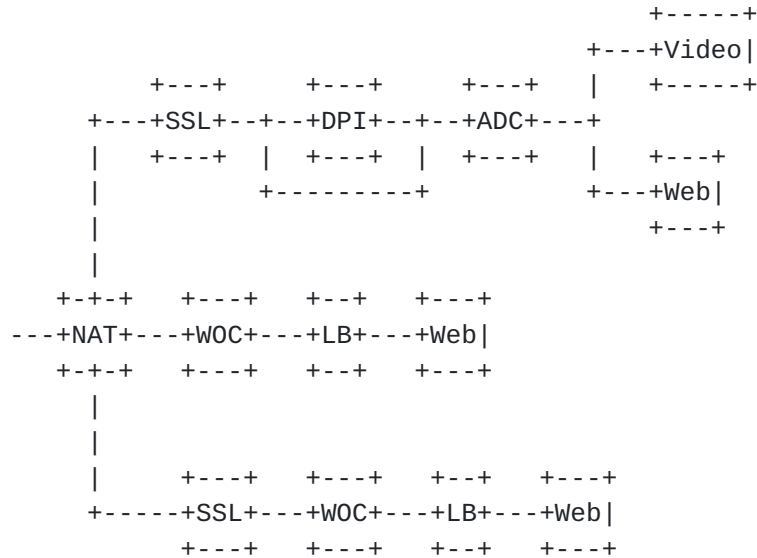
Figure 1 : Service function chains created by Enterprise B.
