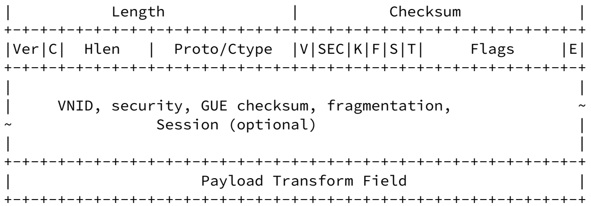
Figure 2 GUE Header with Payload Transform Flag
