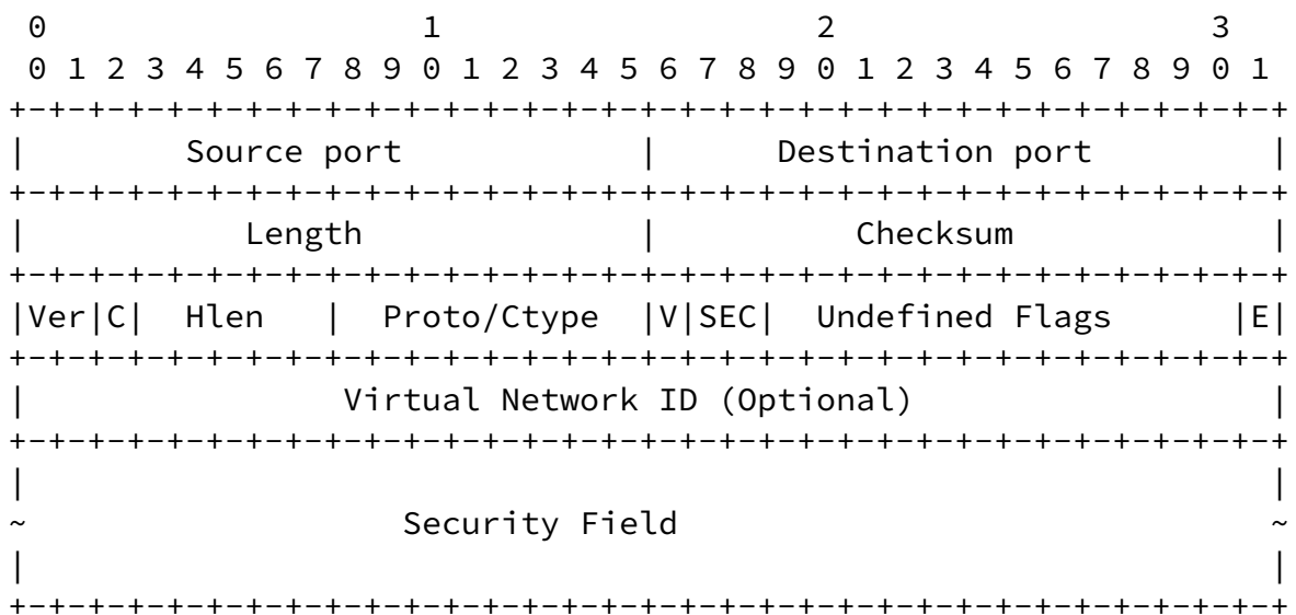
Figure 1 GUE Header Format with Security Flag
