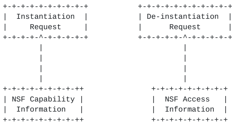
Figure 2: Instance Management Sub-Model
