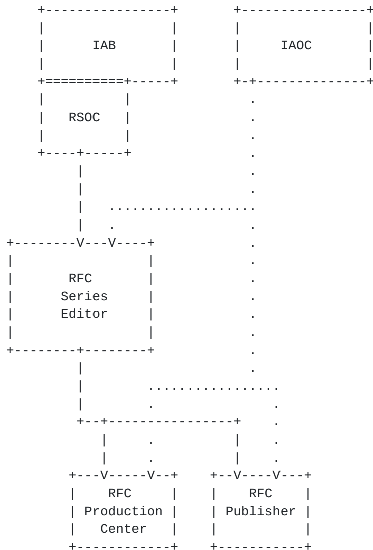
Authority Structure of RFC Series
