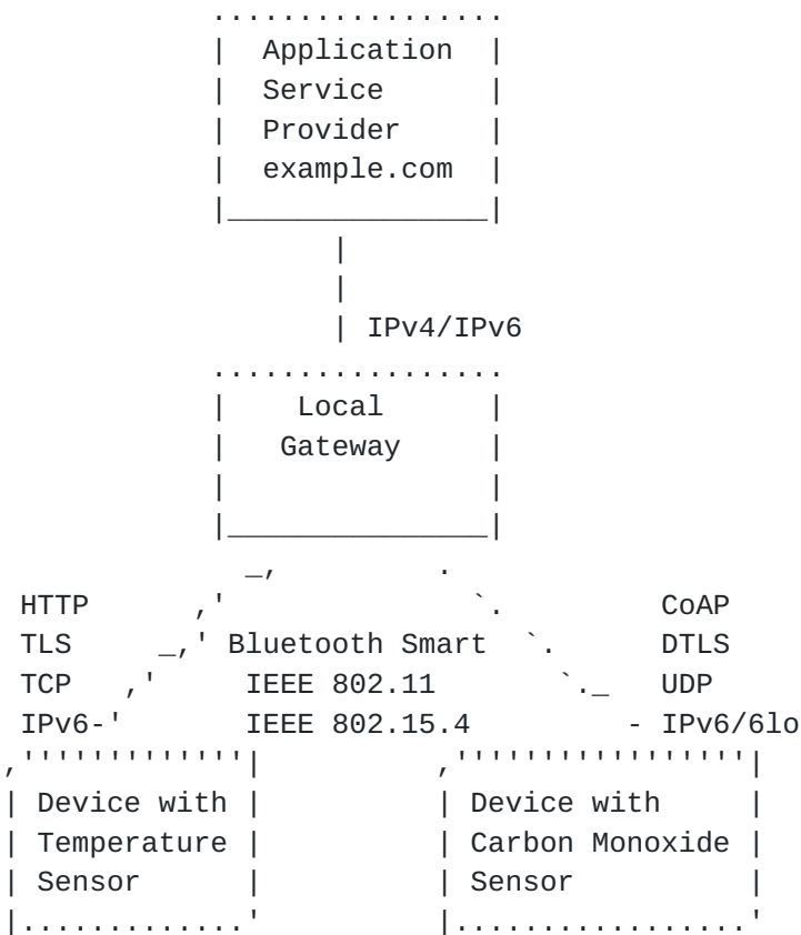
Figure 3: Device-to-Gateway Communication Pattern
