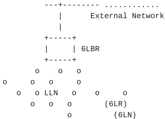
Figure 4: Basic Configuration
