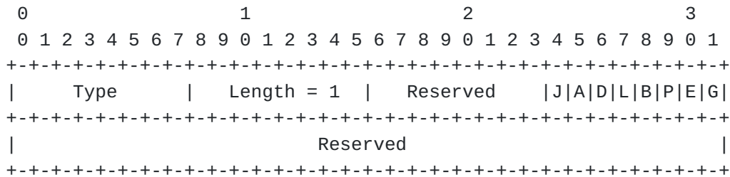
Figure 4: New Capability Bits in the 6CIO
