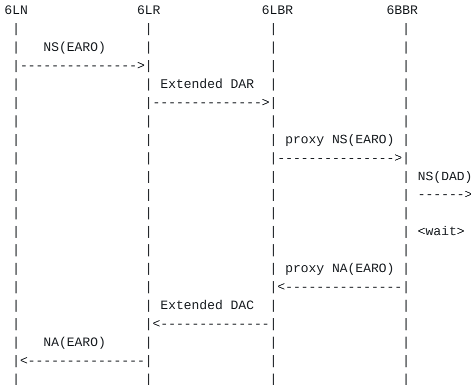
Figure 7: (Re-)Registration Flow
