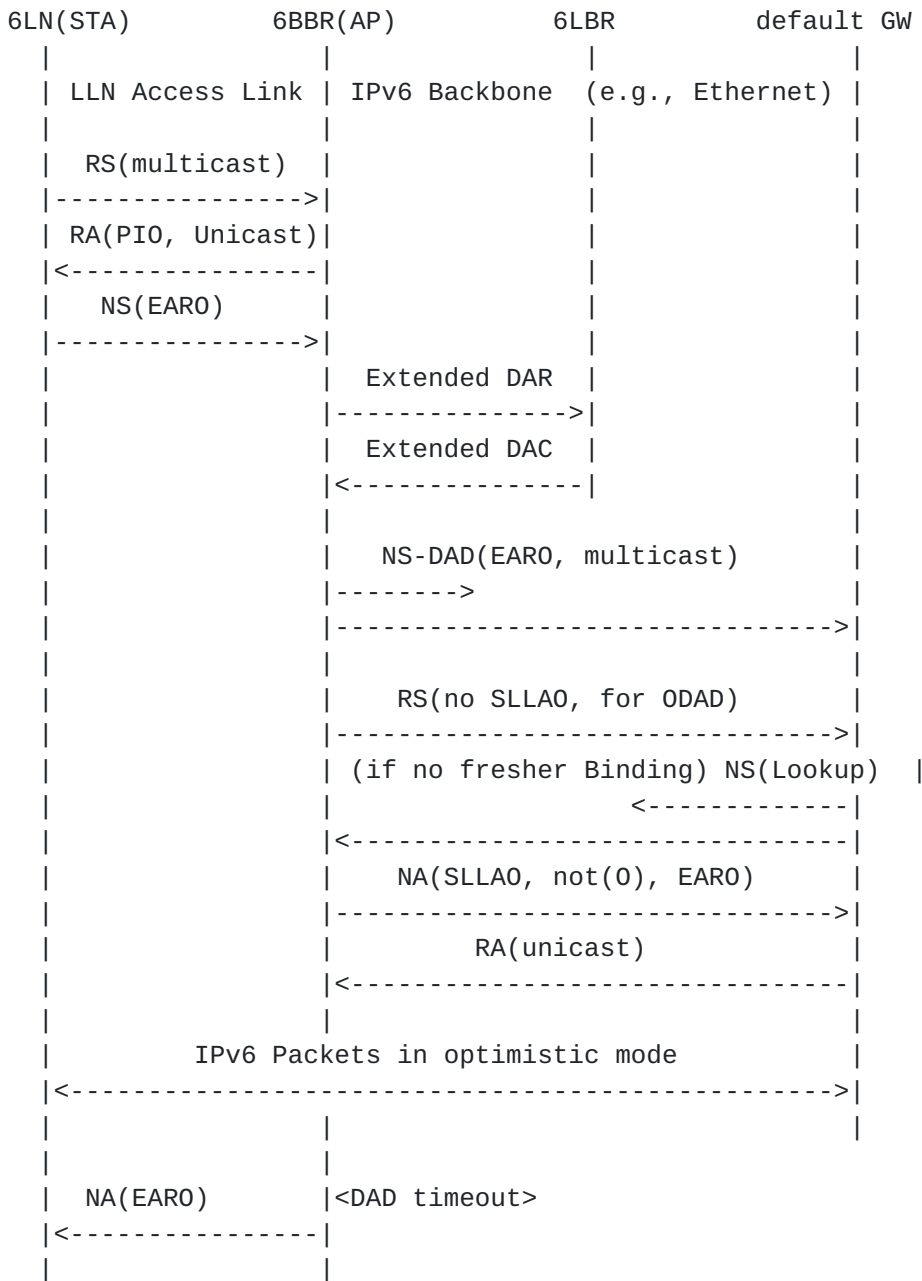
Figure 2: Initial Registration Flow to a 6BBR acting as Routing Proxy
