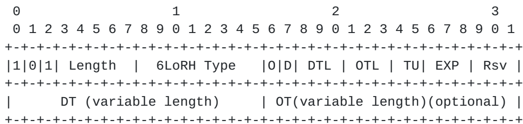
Figure 2: Deadline-6LoRHE format
