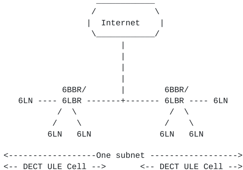
Figure 7: Multiple DECT ULE cells in a single Multi-Link subnet
