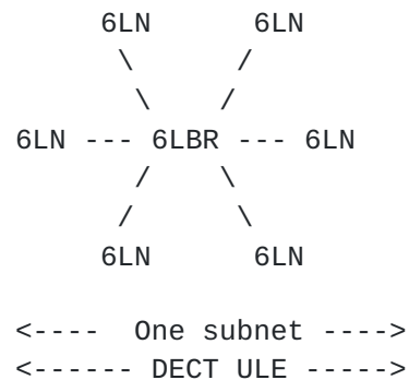
Figure 6: Isolated DECT ULE network
