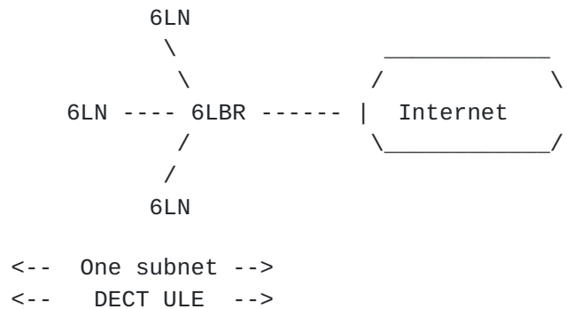
Figure 5: DECT ULE network connected to the Internet
