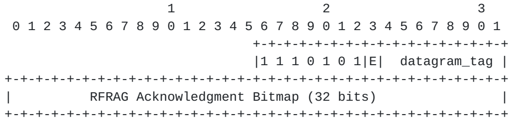
Figure 4: RFRAG Acknowledgment Dispatch type and Header
