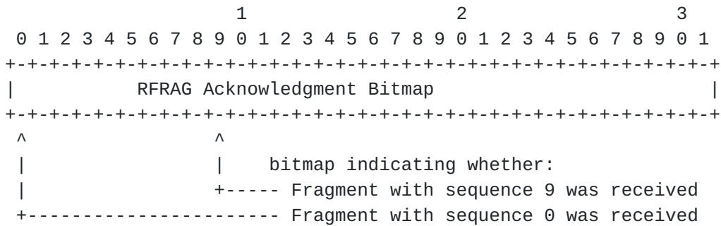
Figure 2: RFRAG Acknowledgment bitmap encoding
